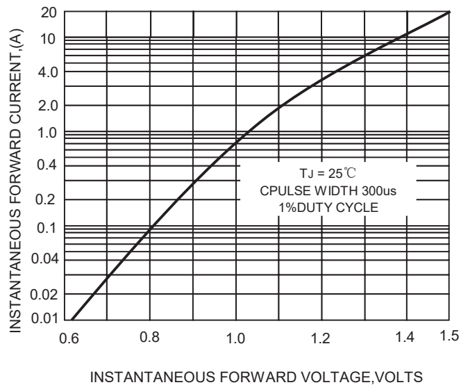
FIG.2-TYPICAL FORWARD CHARACTERISTICS
