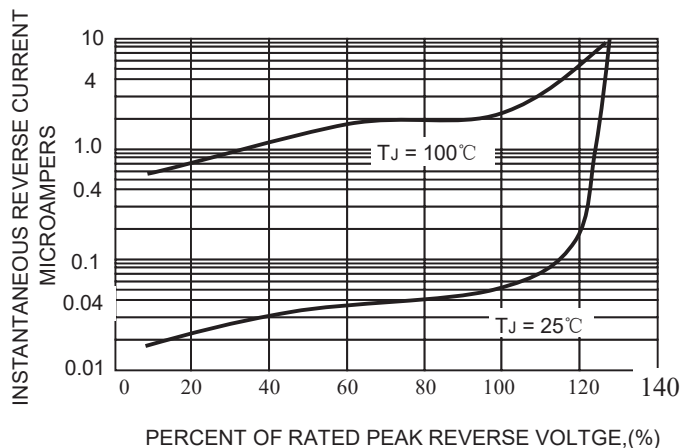
FIG.6-TYPICAL REVERSE CHARACTERISTICS
